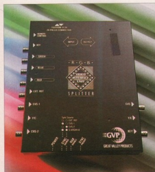
A close look at the long-awaited IV24 splitter, (labelling with inputs and outputs, as all the best add-ons should)
